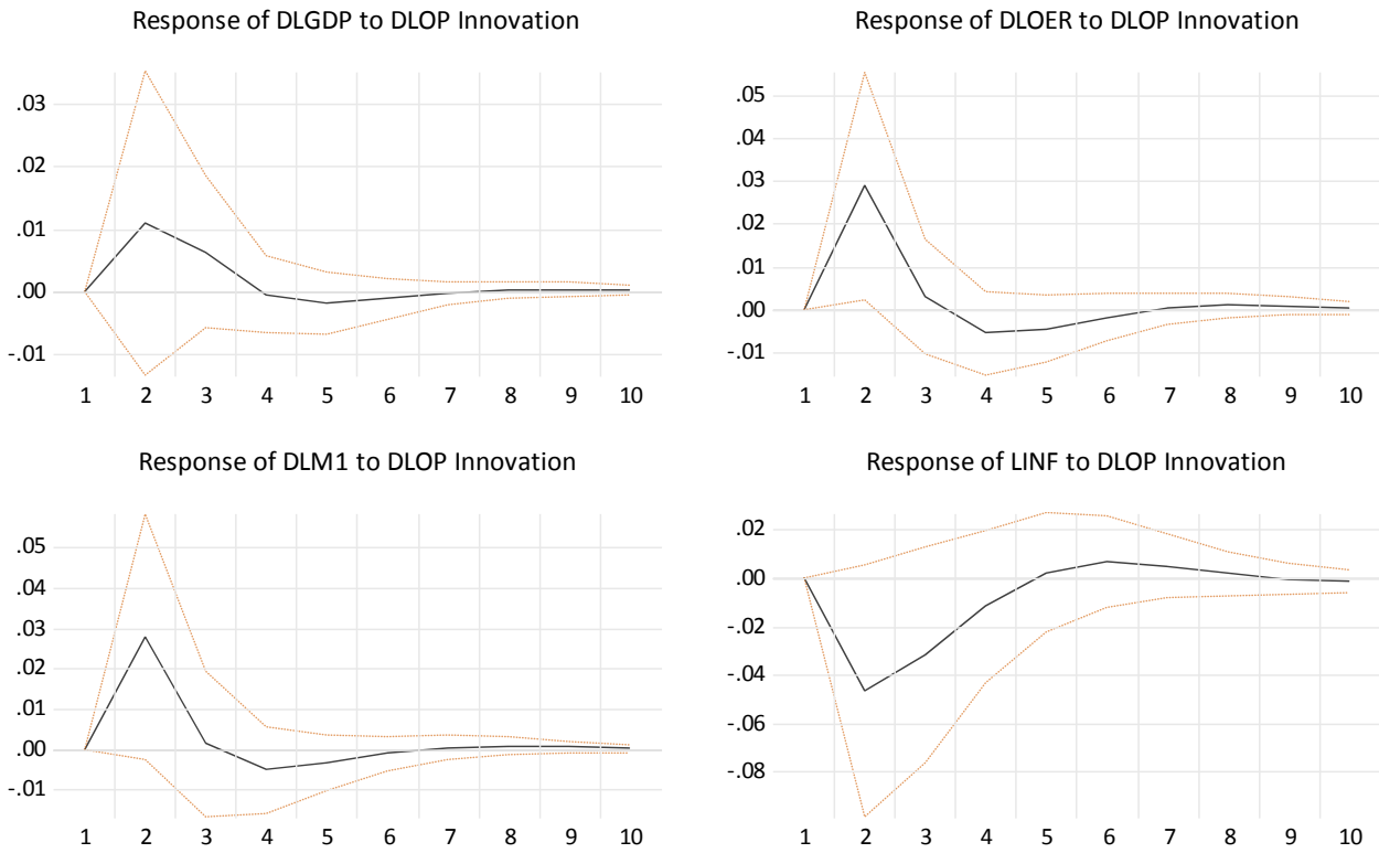
Figure 2: Response to Cholesky One S.D. Innovations \pm 2 S.E.s
